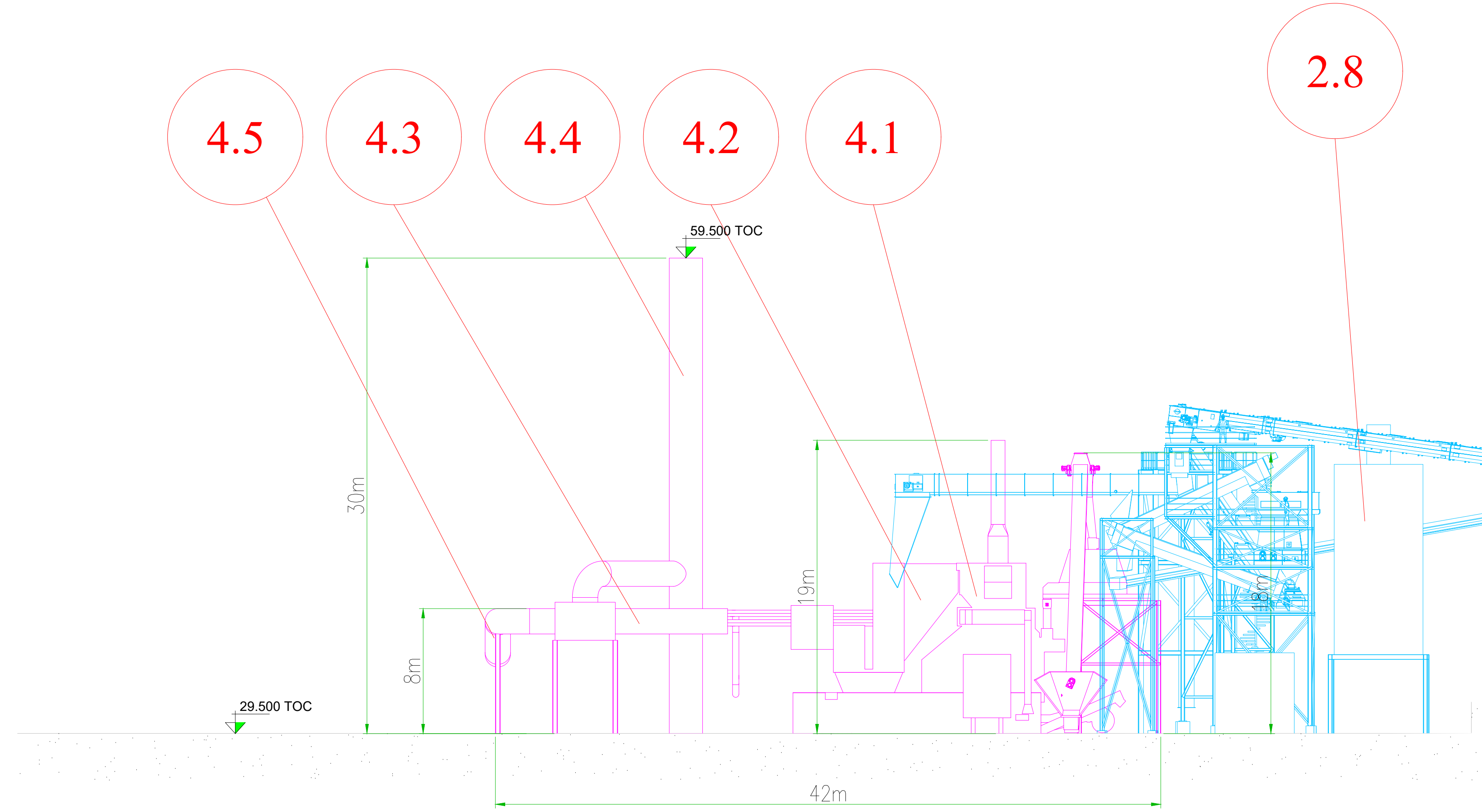
Section B-B
