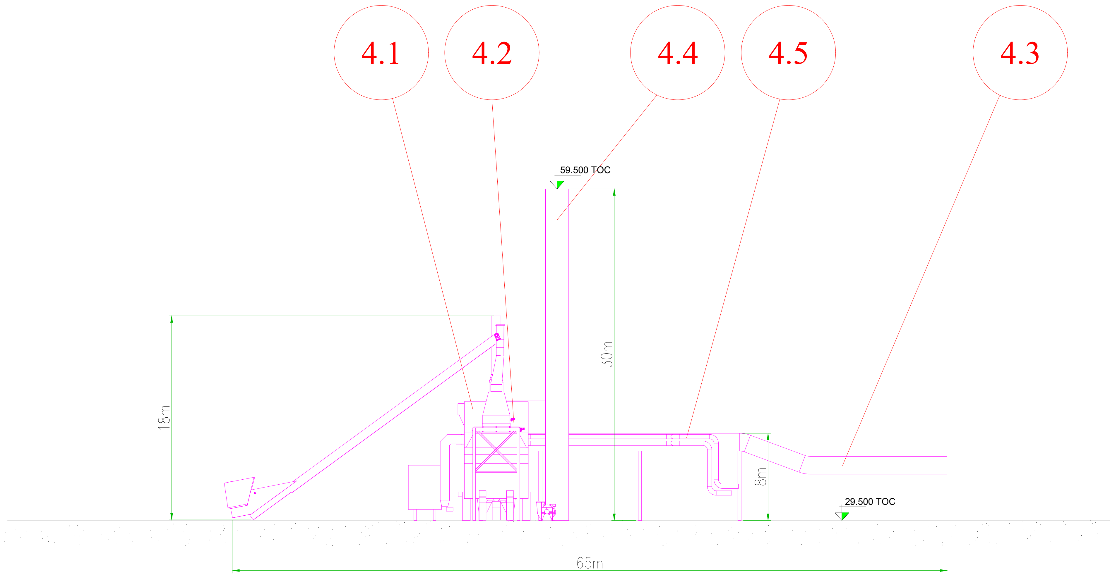
Section C-C
